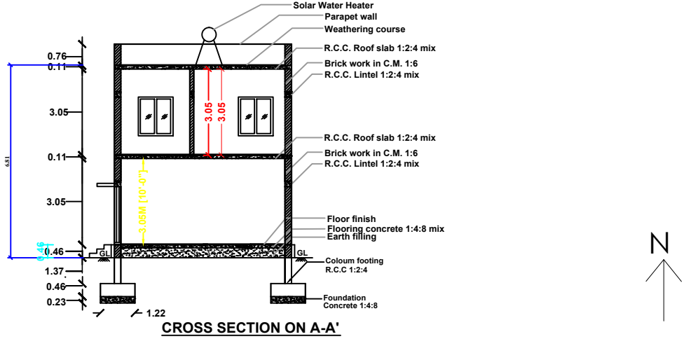
CROSS SECTION ON A-A'
