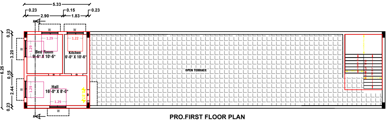
PRO.FIRST FLOOR PLAN
