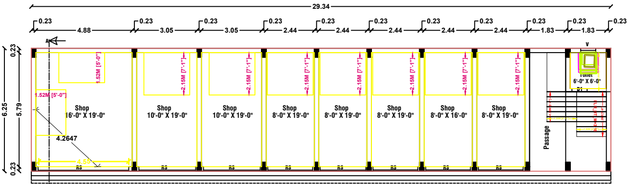
EXI.GROUND FLOOR PLAN
