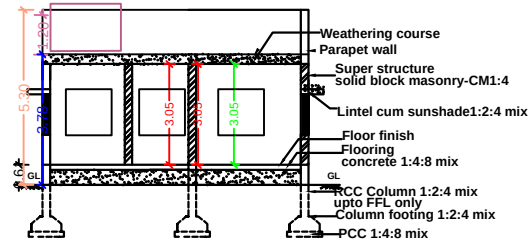
SECTION ELEVATION
