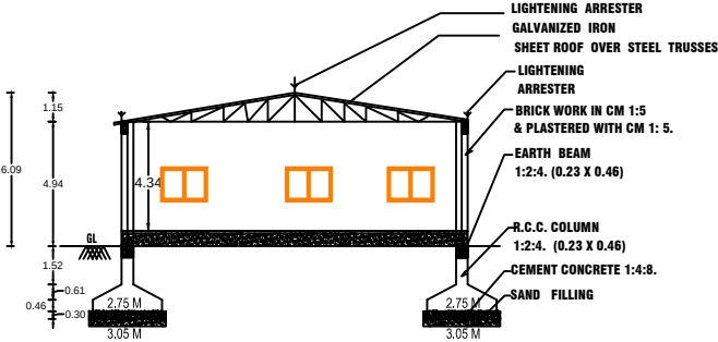
SCETION ON 'A-B'
