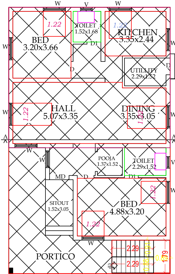
EXG. GROUND FLOOR
