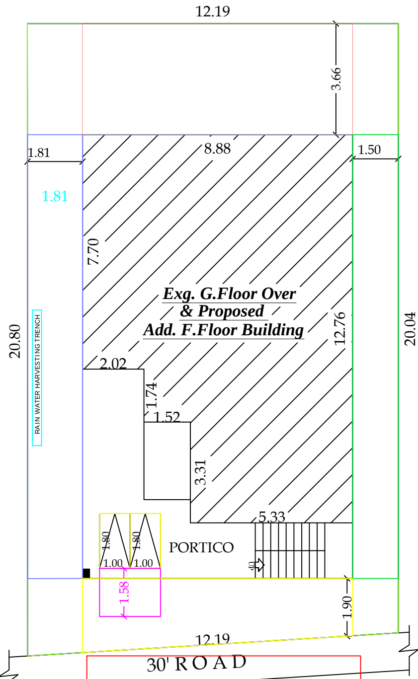
SITE PLAN
