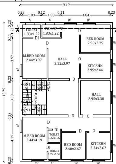
PRO.T.FLOOR PLAN
