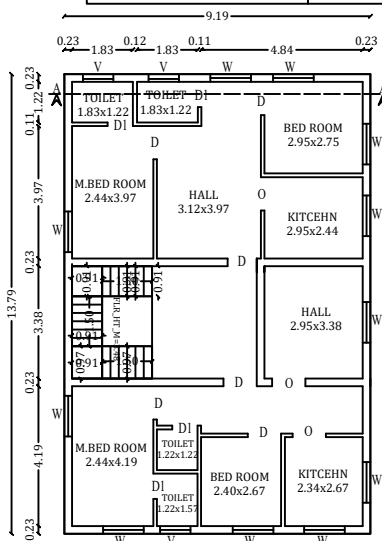
PRO.S.FLOOR PLAN
