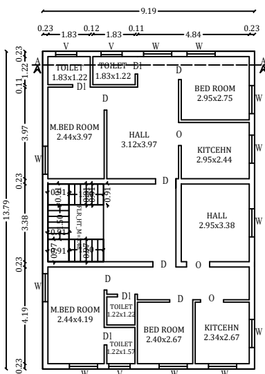
PRO.F.FLOOR PLAN
