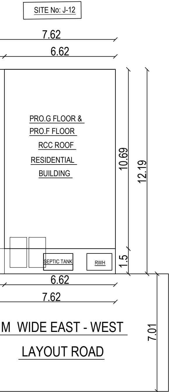
SITE PLAN
