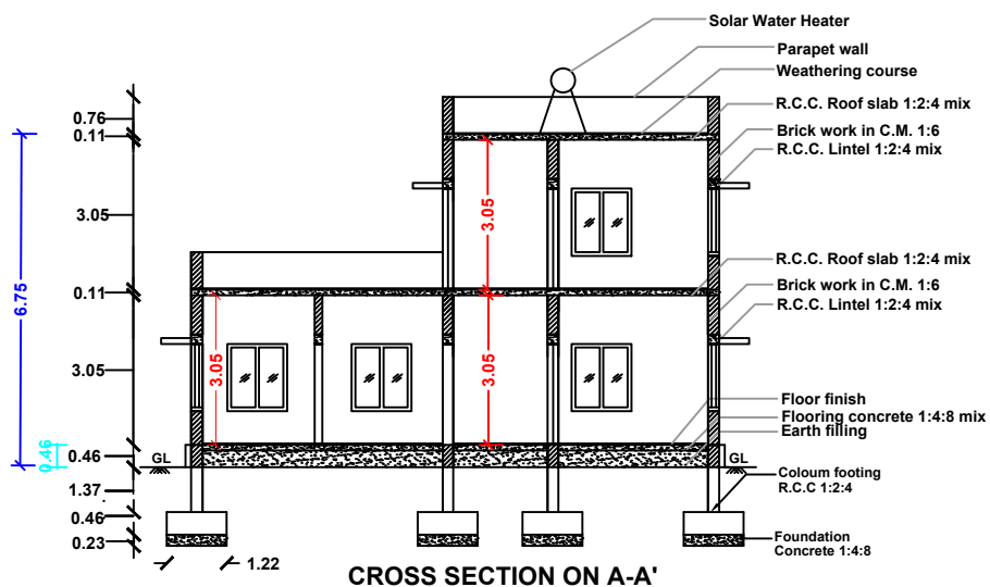
CROSS SECTION ON A-A'
