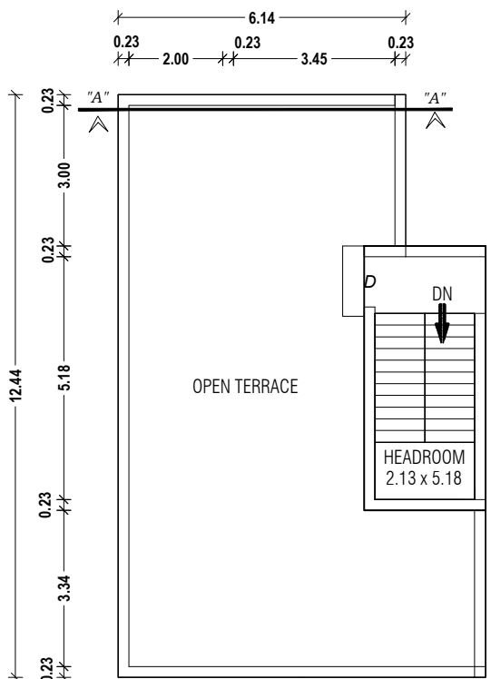
PRO. TERRACE FLOOR PLAN
