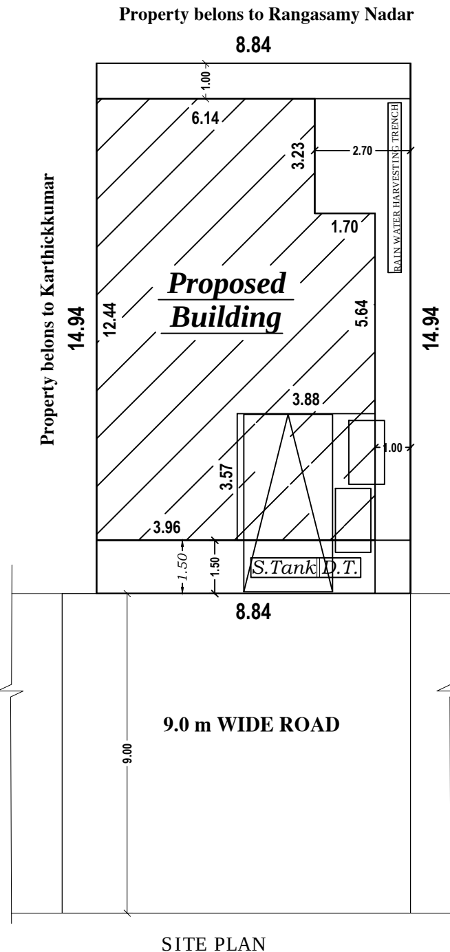
SITE PLAN
