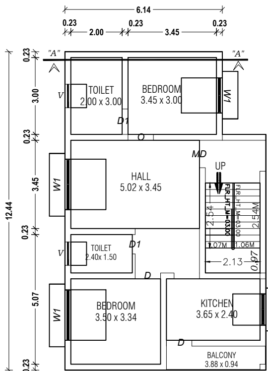
PRO. FIRST FLOOR PLAN
