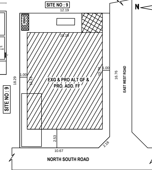
SITE PLAN
