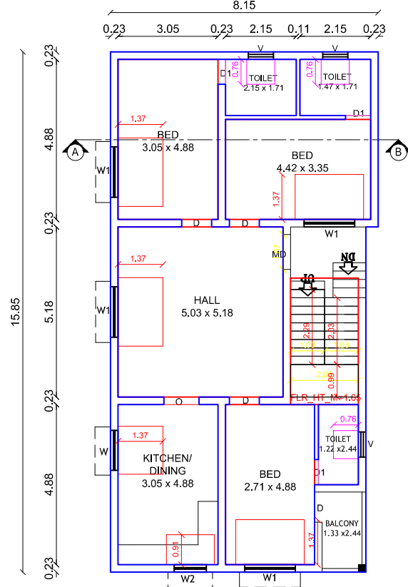
PRO.ADDL.FIRST FLOOR PLAN
