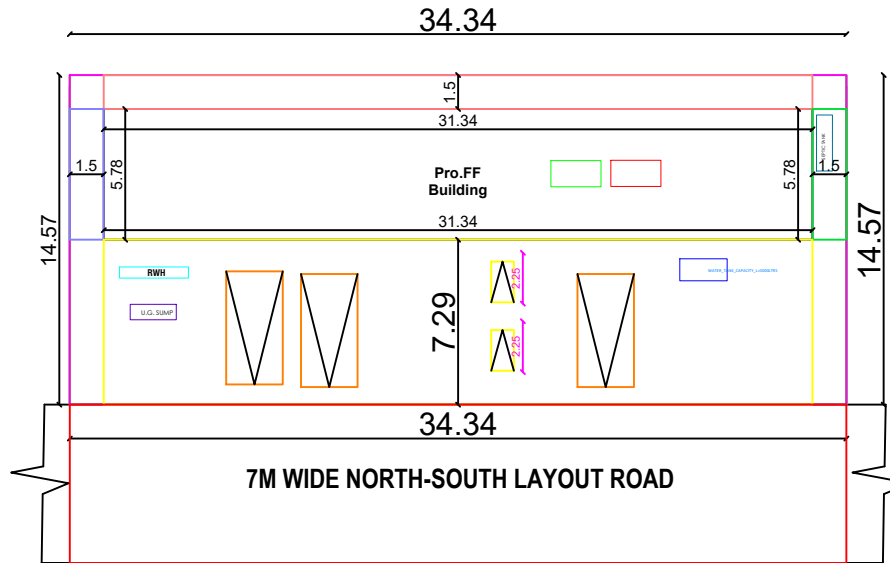
SITE PLAN (SCALE 1" : 8' 0")
