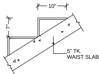
STAIRCASE SECTION (NOT TO SCALE)
