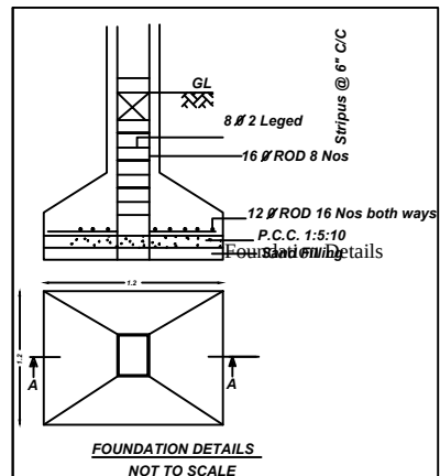
FOUNDATION DETAILS NOT TO SCALE
