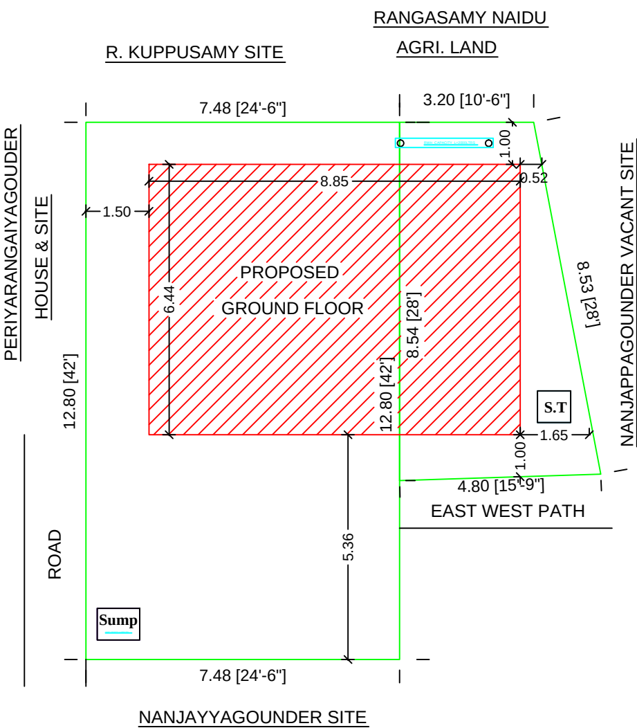
SITE PLAN
