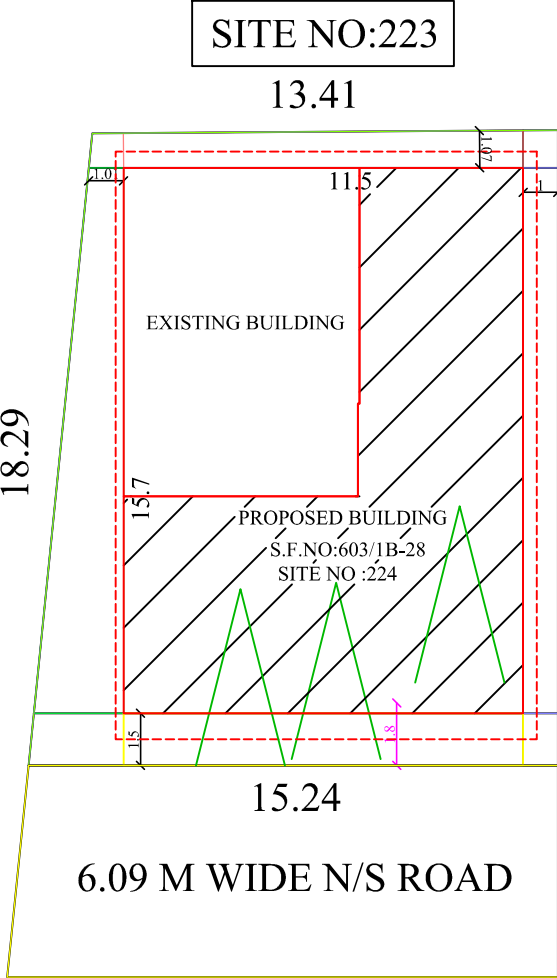
SITE PLAN
