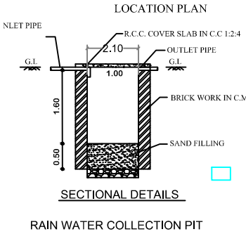
RAIN WATER COLLECTION PIT
