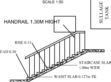
STAIRCASE DETAILS
