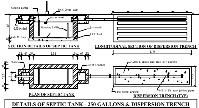
DETAILS OF SEPTIC TANK - 250 GALLONS & DISPERSION TRENCH
