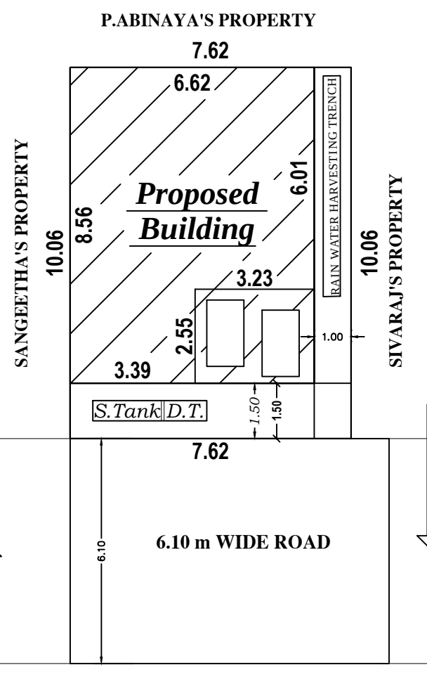
SITE PLAN
