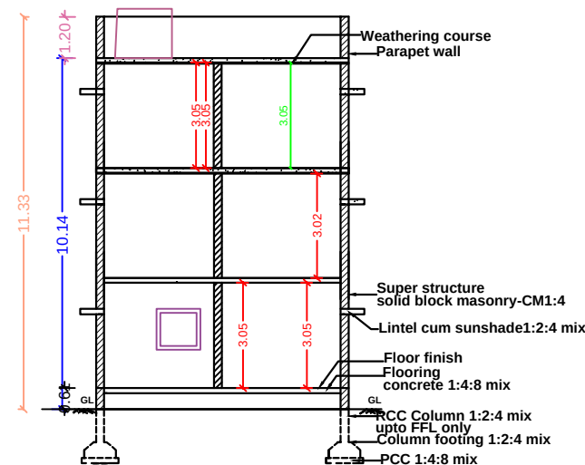
SECTION ELEVATION
