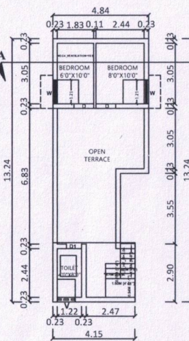
PRO. SECOND FLOOR
