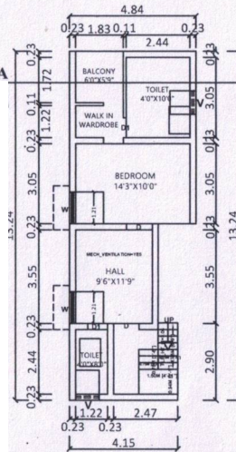
PRO. FIRST FLOOR
