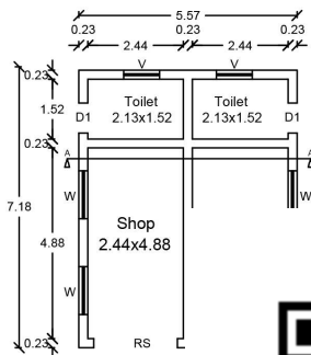
GROUND F
