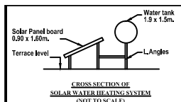
CROSS SECTION OF SOLAR WATER HEATING SYSTEM (NOT TO SCALE)
