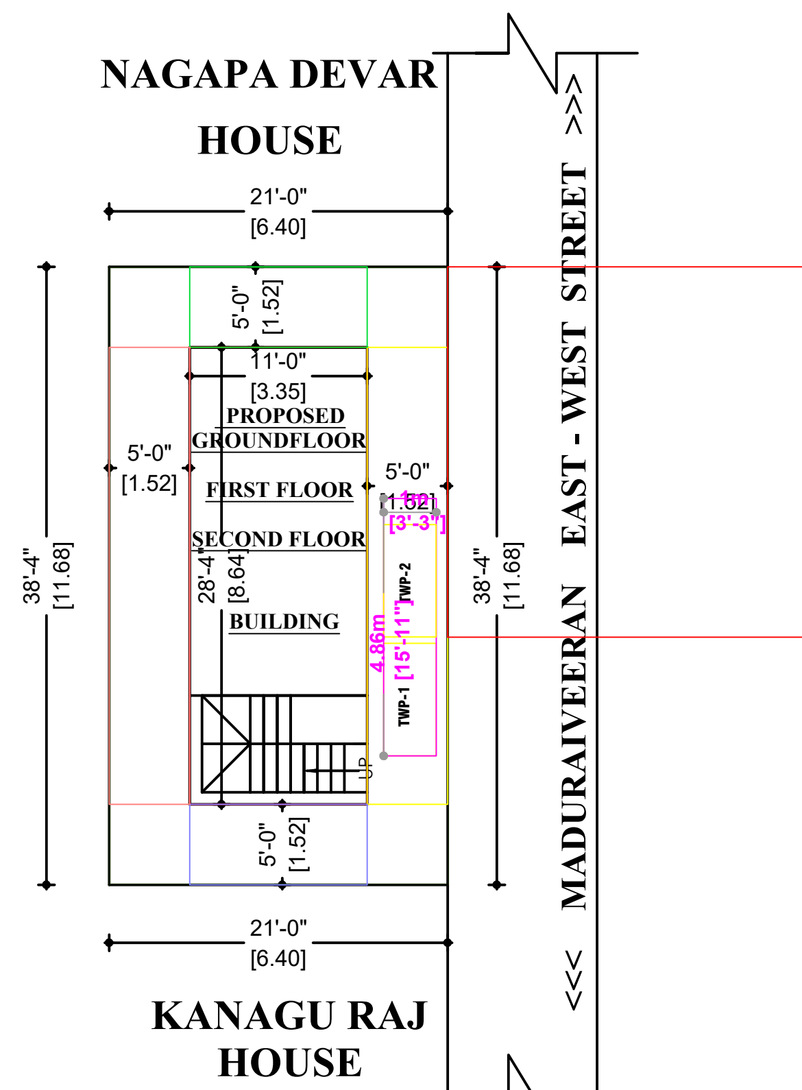
SITE PLAN
