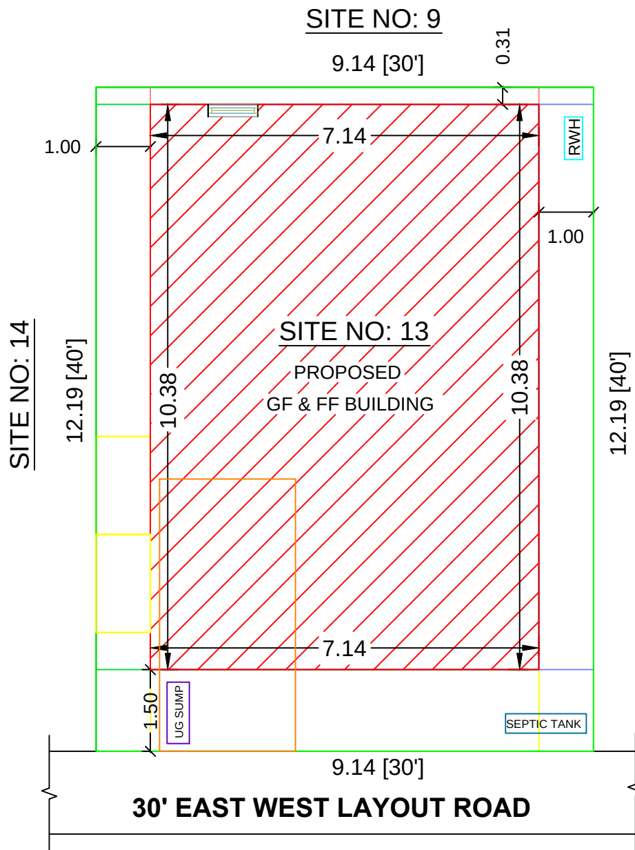
SITE PLAN
