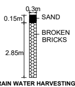
RAIN WATER HARVESTING DETAILPERCOLATION PIT (NTS)
