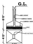
FOUNDATION DETAILS (NOT TO SCALE)
