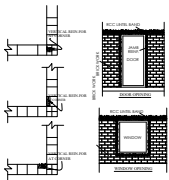
EARTHQUAKE SAFE DESIGN (NOT TO SCALE)
