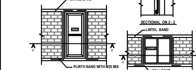
Figure - 2 Reinforcement and Detailing Details of Seismic Bands.
