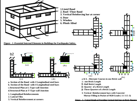
Figure - 1 Essential Elements in Buildings for Earthquake Safety.
