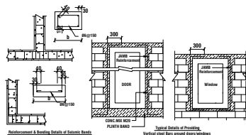
Essential Internal Elements in Buildings
