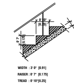
STAIRCASE DETAILS:
