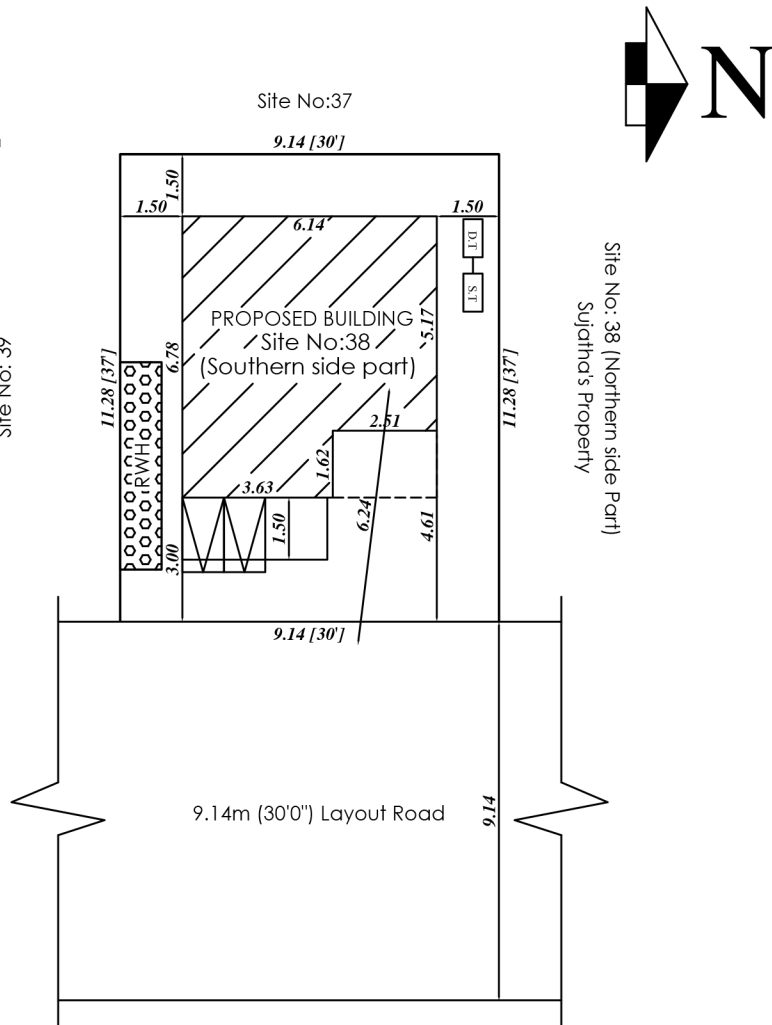
Site Plan
