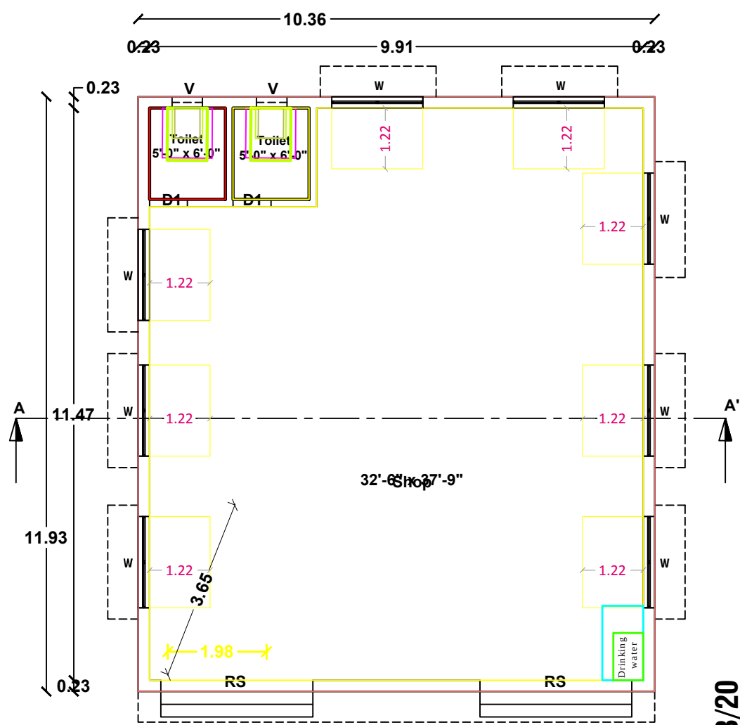
FLOOR PLAN
