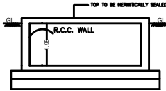
RWH SECTION (SAMPLE) RWH_CAPACITY_L=2000LTRS
