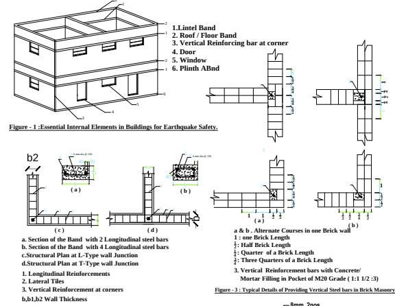
Figure - 1: Essential Internal Elements in Buildings for Earthquake Safety.
