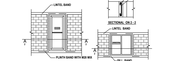
Figure - 2: Reinforcement and Detailing Details of Seismic Bands.
