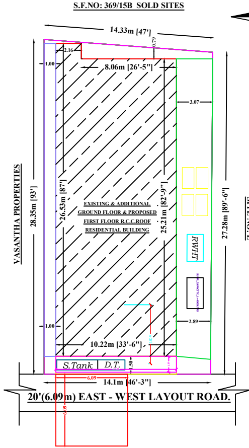
SITE PLAN
