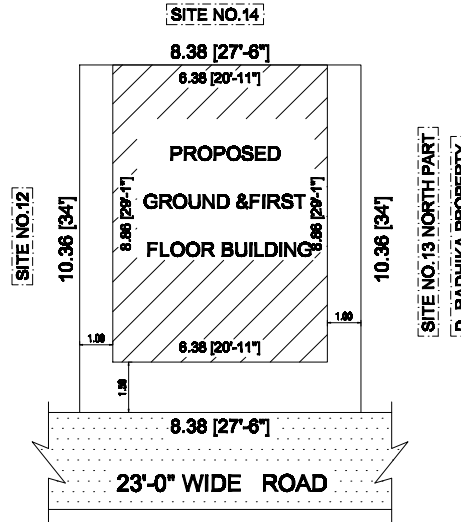
SITE PLAN
