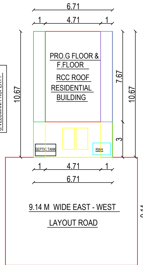
SITE PLAN
