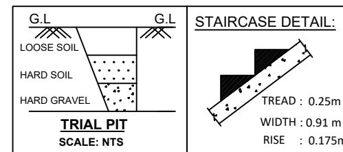
STAIRCASE DETAIL:
