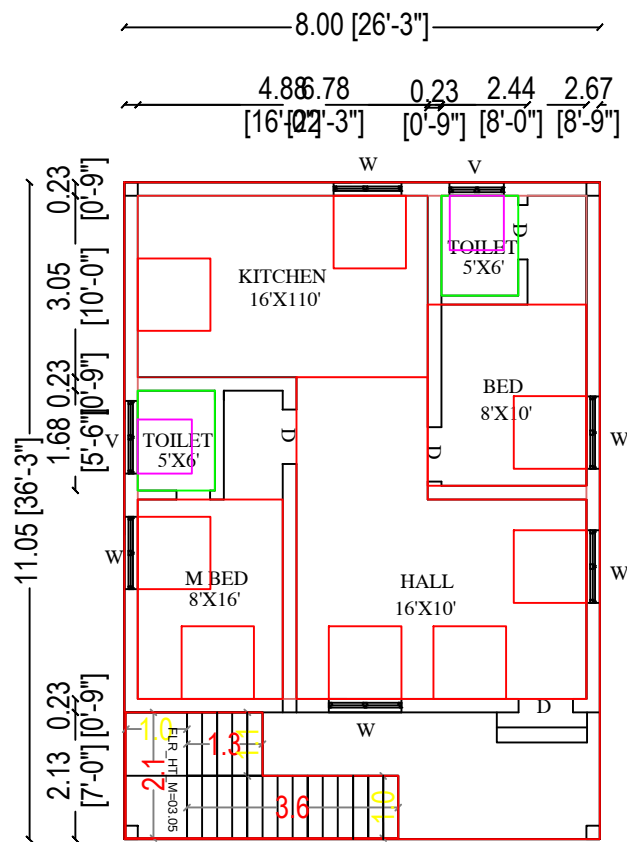
PROPOSED PLAN
