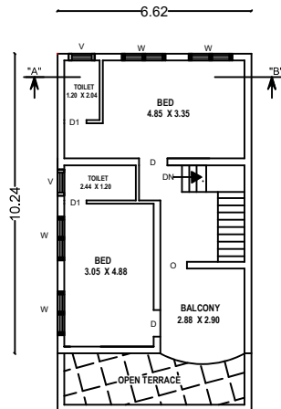
PRO.F.F. PLAN
