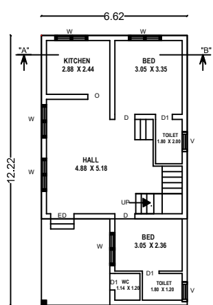
EXG.G.F. PLAN
