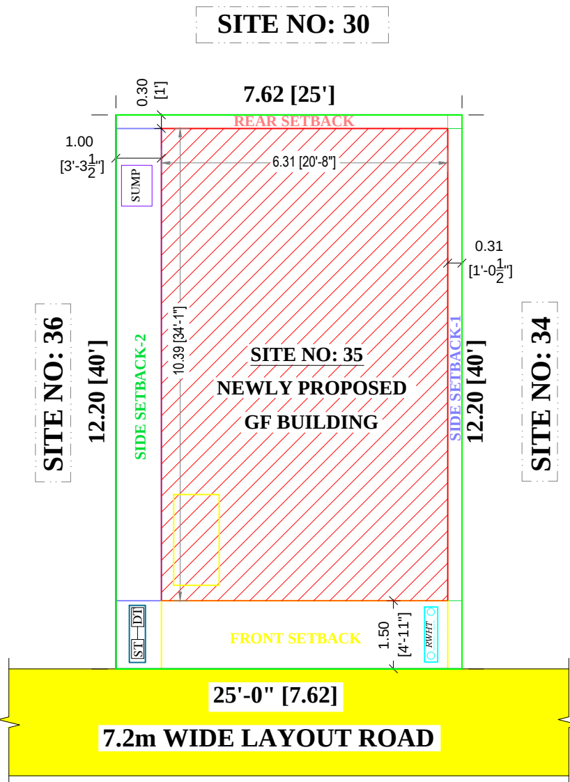
SITE PLAN
