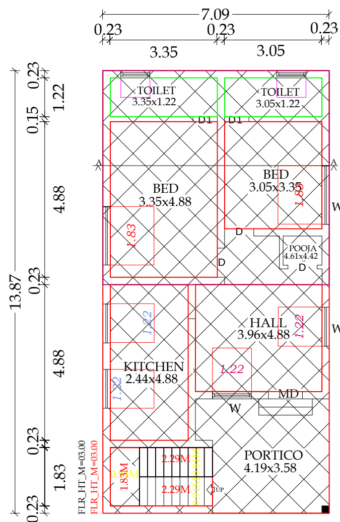
EXG. GROUND FLOOR PLAN
