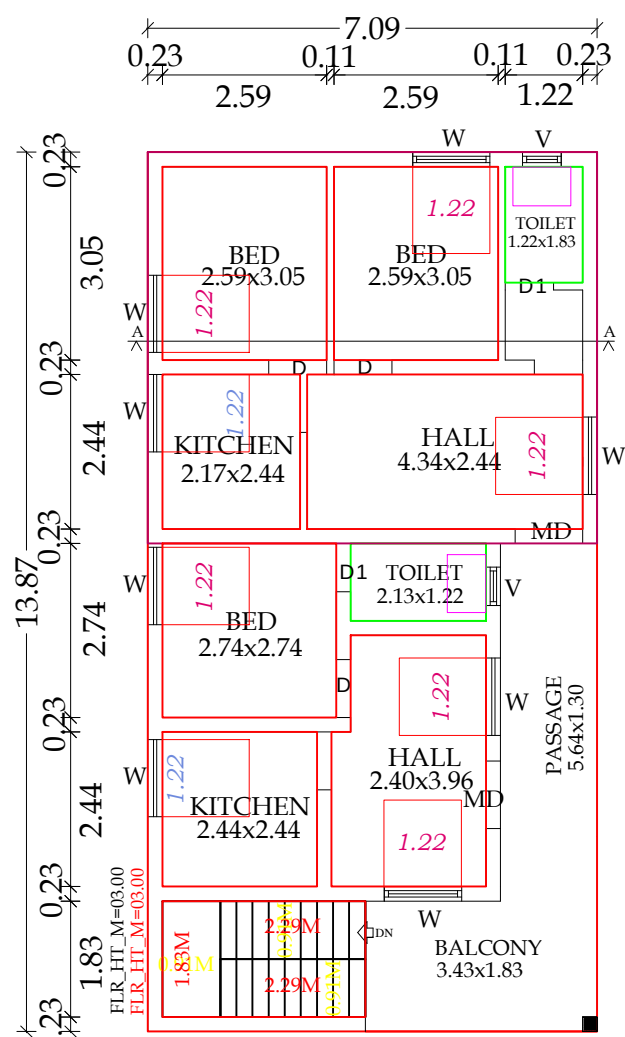
PRO. ADD. FIRST FLOOR PLAN
