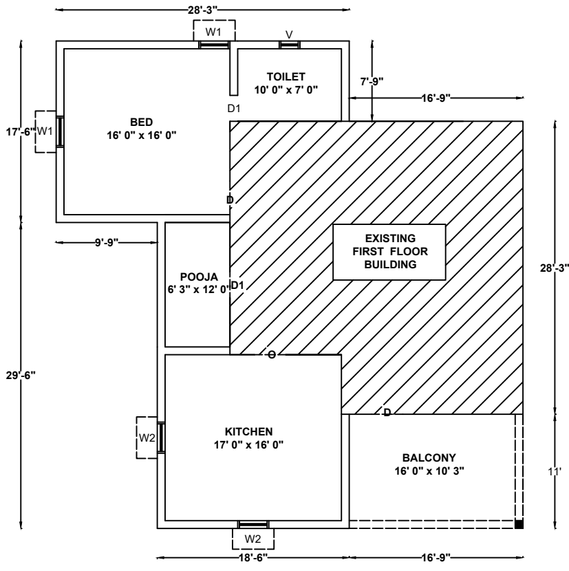
FIRST FLOOR PLAN - EXTENSION
