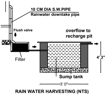
RAIN WATER HARVESTING (NTS)
