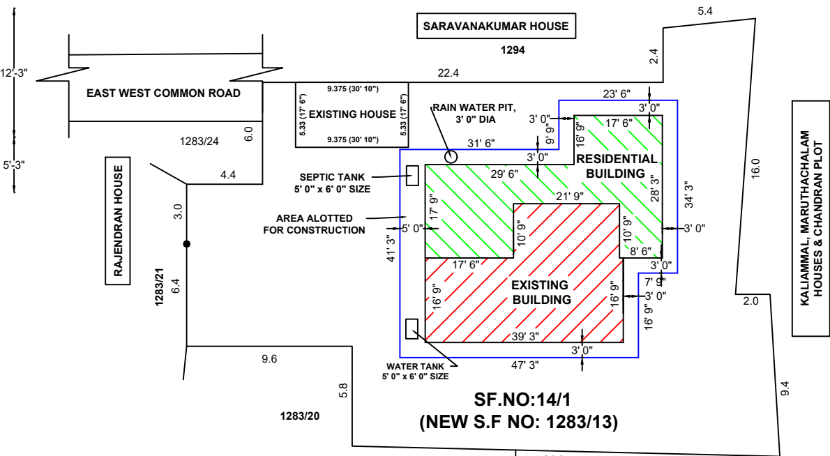
SITE PLAN
