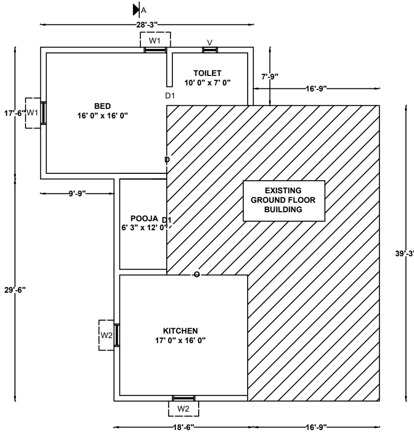
GROUND FLOOR PLAN - EXTENSION
