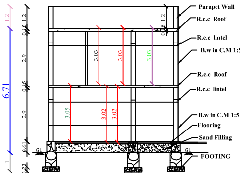
SECTION AB
