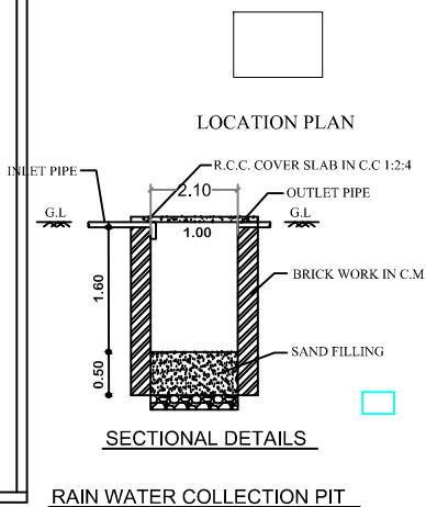
RAIN WATER COLLECTION PIT
