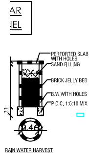
RAIN WATER HARVEST
