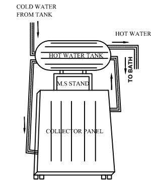
SOLAR WATER HEATER SYSTEM
