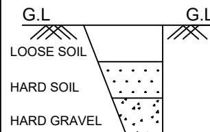
TRIAL PIT SCALE: NTS
