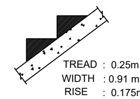
STAIRCASE DETAIL:
