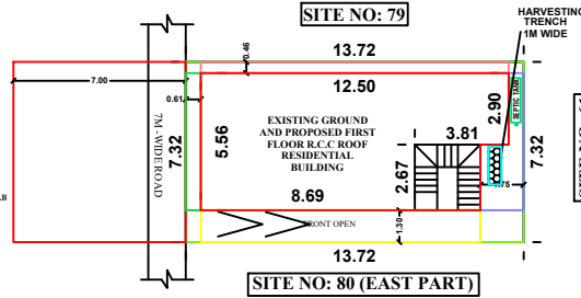
SITE PLAN
