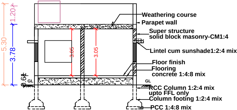
SECTION ELEVATION
