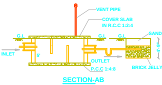
SECTION-AB
