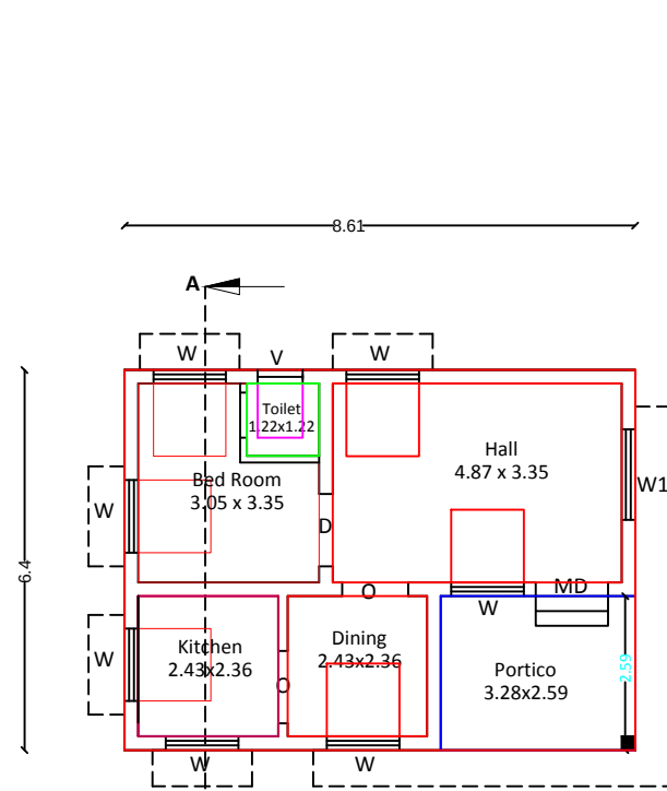
3F PLAN
