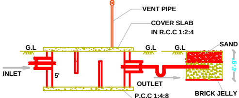
SECTION-AB
