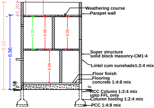
SECTION ELEVATION
