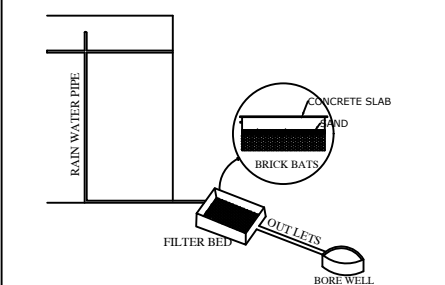
RAIN WATER HARVESTING TANK
