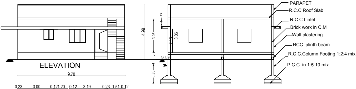
SECTION ON A-A RAYAPPAN'S PROPERTY
