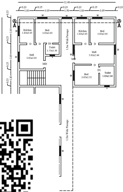
PLAN
