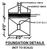
FOUNDATION DETAILS (NOT TO SCALE)
