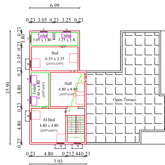
Plan for Proposed First Floor
