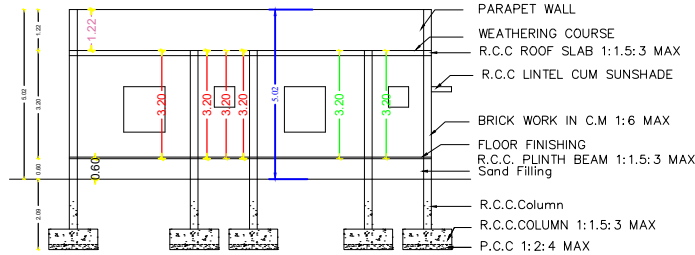
SECTION
