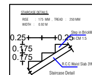
Staircase Detail
