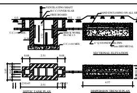
SEPTIC TANK DISPERSION TRENCH 450 GALLONS
