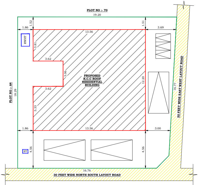
SITE PLAN
